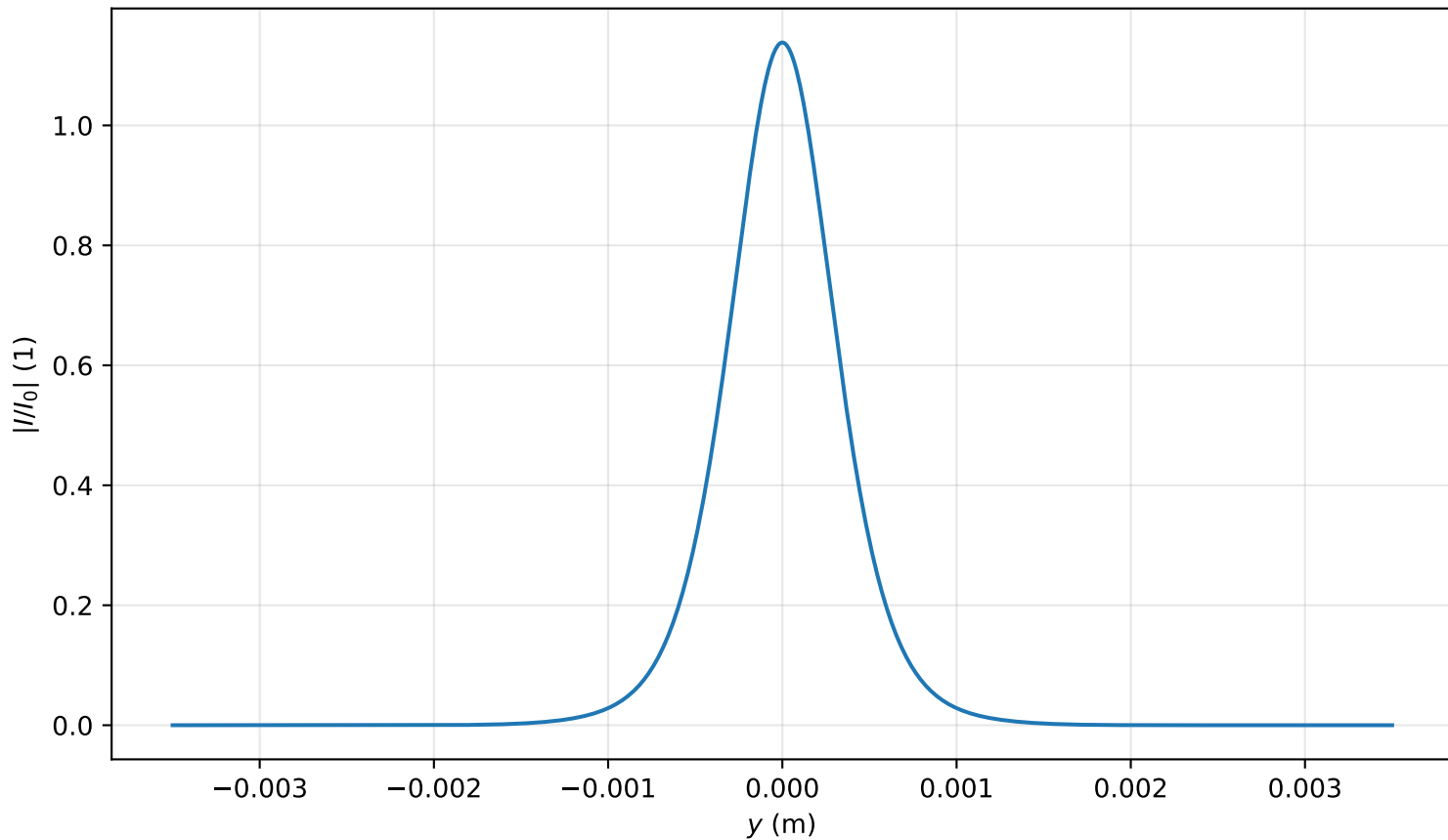
Intensity profile I(x=0, y, z=1.831)/I_0 , P_{in}=0.7P_{cr} , artificial time
